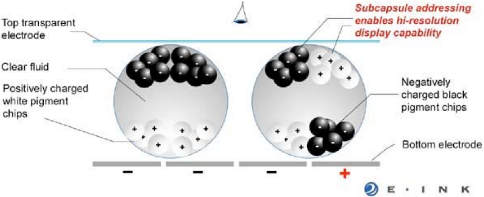
Cross-Section of Electronic-Ink Microcapsules
