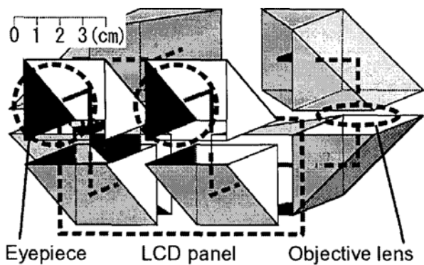
Figure 18. A compact optics design of the display.
