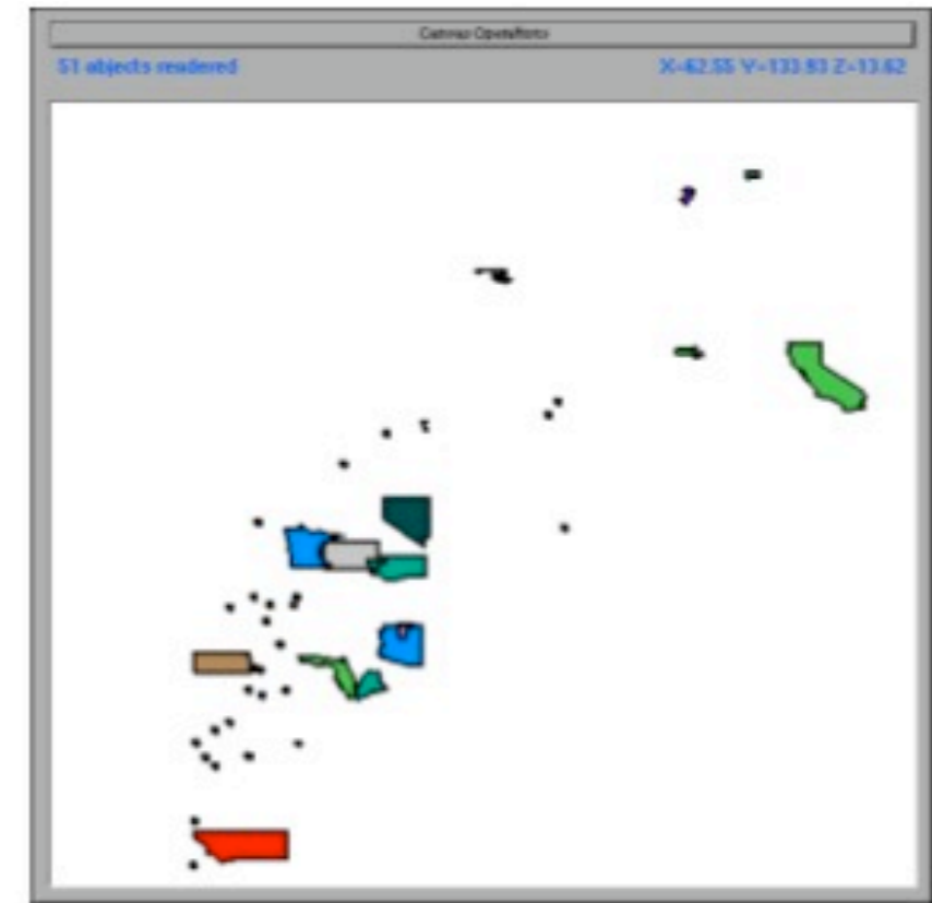
Figure 1c: VIDA visualization.
