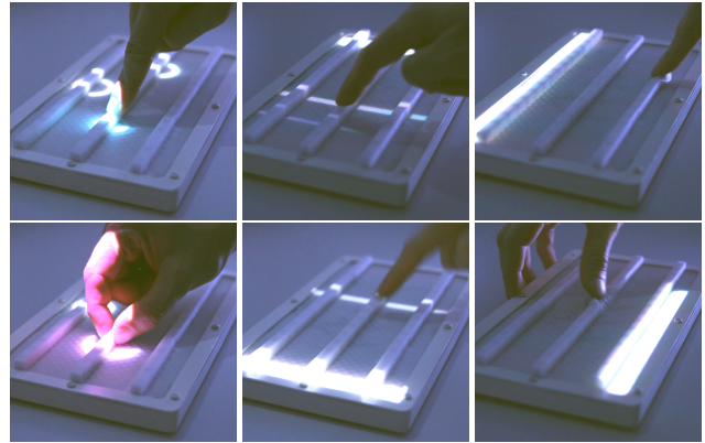
Figure 7: StringTouch offers the following interactions: push/pull (l.), swipe left/right (m.), strum down/up (r.). Feedback is designed with high-contrast to enable interaction with little visual attention.
