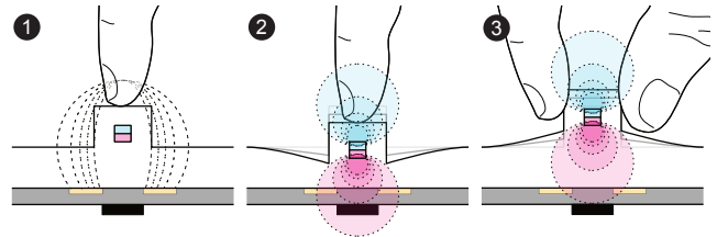
Figure 9: ① Without deformation, a finger increases the capacitance. Further, ② pushing reduces the distance between magnet and sensor (hall effect: high V), while ③ pulling increases the distance (low V).
