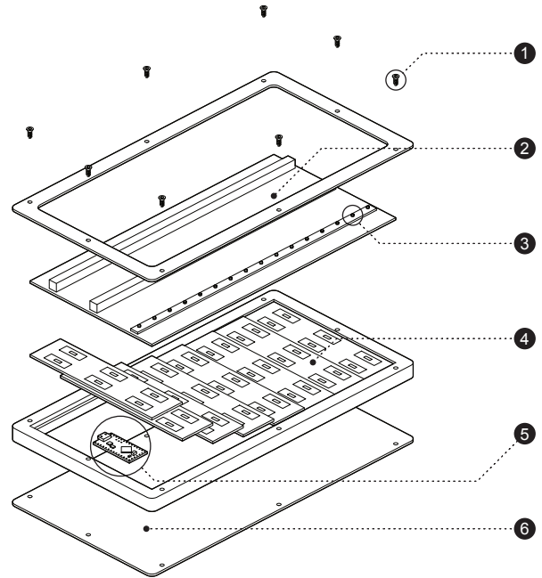
Figure 8: ① Screws ② Silicone interaction surface ③ Magnets ④ PCBs ⑤ Teensy LC ⑥ Enclosure
