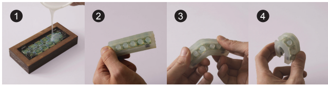
Figure 12: ❶ The PCB is embedded in the silicone cast. ❷ The unbroken sensor is rigid. After ❸ breaking, it can easily be ❹ bent. Such sensor can be used in non planar interfaces such as freely shaped design objects.
